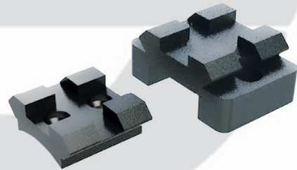
CARRIL VERNEY-CARRON MOUNT VERNEY CARRON EMBASE VERNEY-CARRON Acero, 2 piezas 06.010/00 IPC Acero
